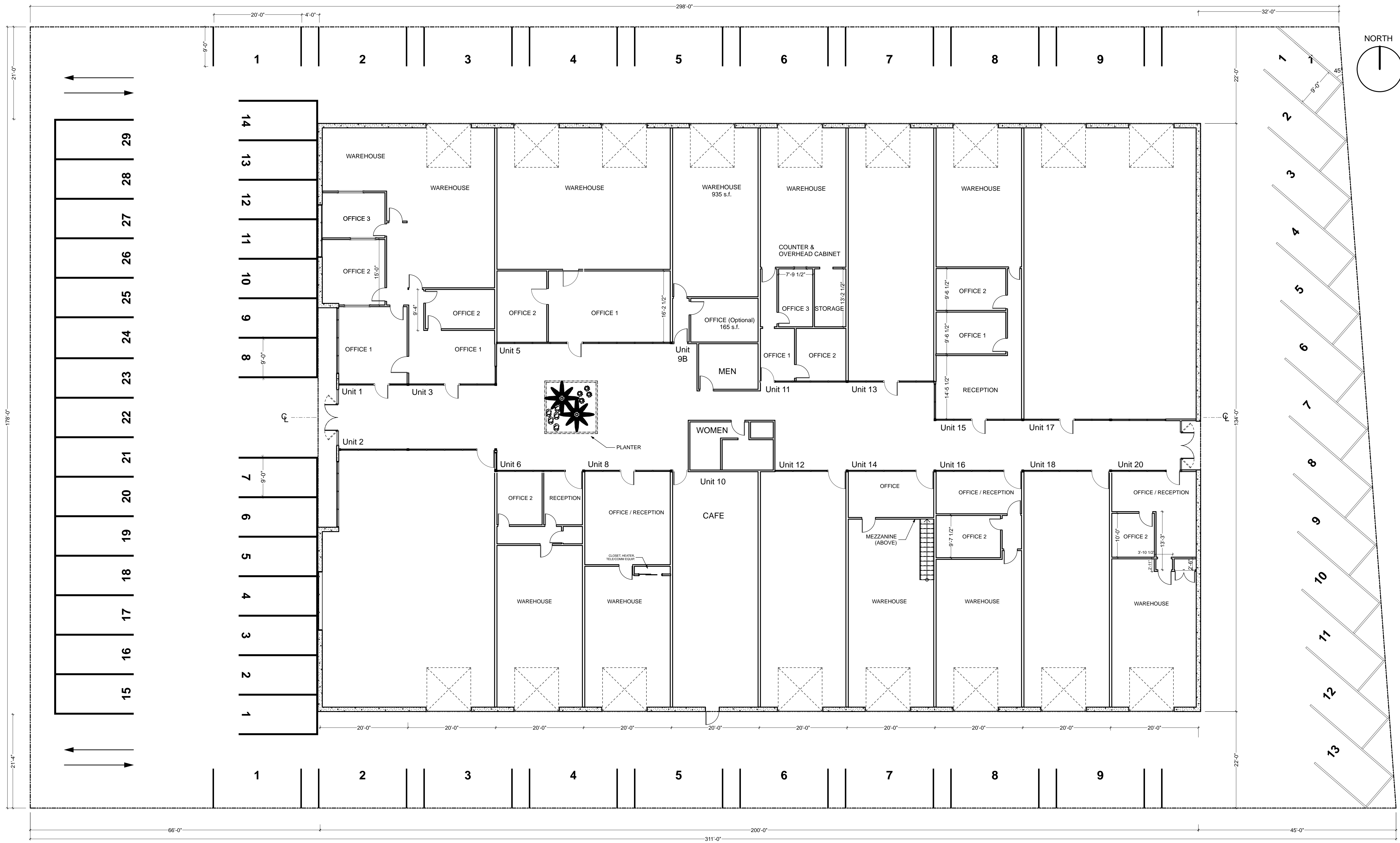
1 FIRST FLOOR PLAN SCALE: 3/32" = 1'-0"
